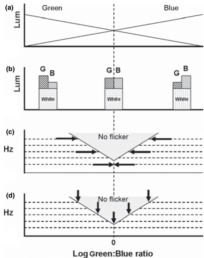
Figure 1. (a) The luminance of the blue and green light emitting diodes (LEDs) are yoked so that there is no change in mean luminance across the range of green-blue ratios; (b) Luminance profiles at different green-blue ratios, illustrating the white pedestal; (c) Conventional heterochromatic flicker photometry (HFP) where subjects adjust green-blue ratio for minimal flicker using a constant flicker rate; (d) method used in current study where flicker rate is gradually reduced and subject presses a button when they detect flicker.
